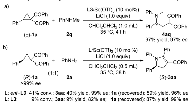
Scheme 1. a) Using a secondary amine as the substrate. b) Control experiments.
